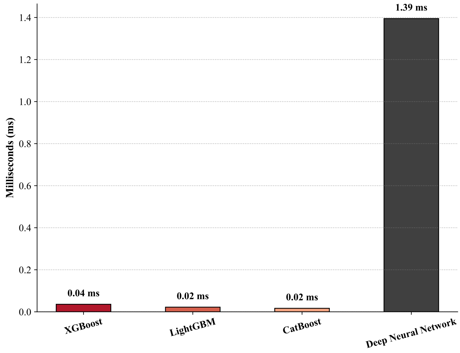
Phase X: Inference Latency (per 1,000 samples)
